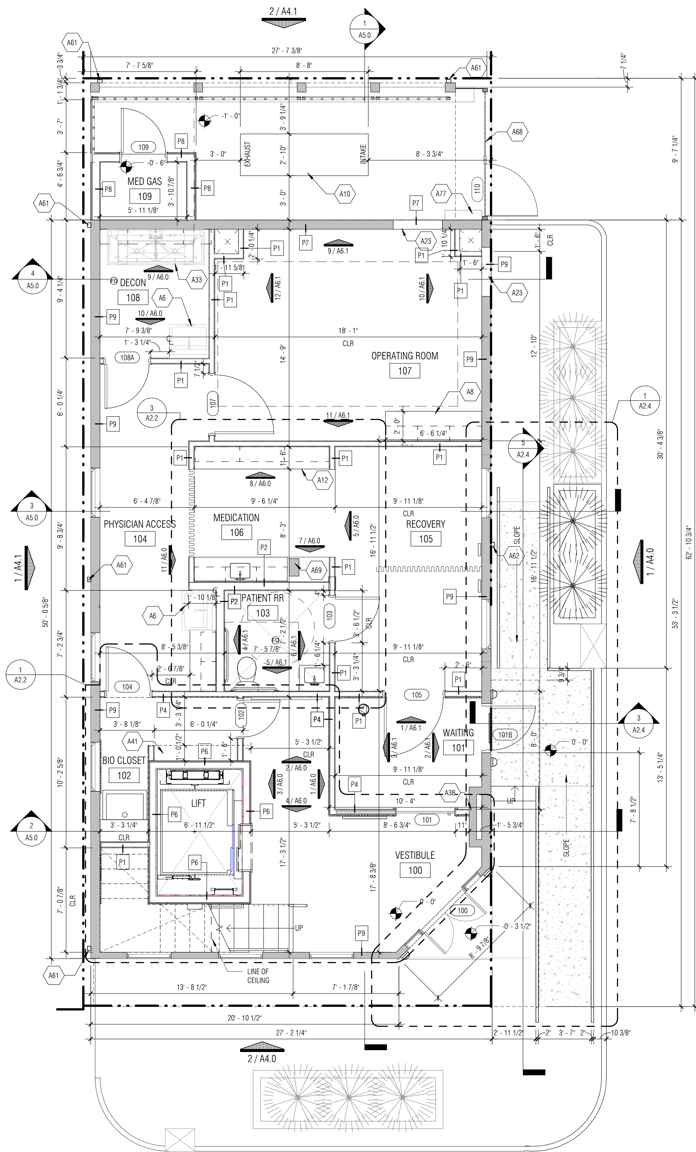
1 | A2.1 | FIRST FLOOR PLAN 1/4" = 1'-0"
