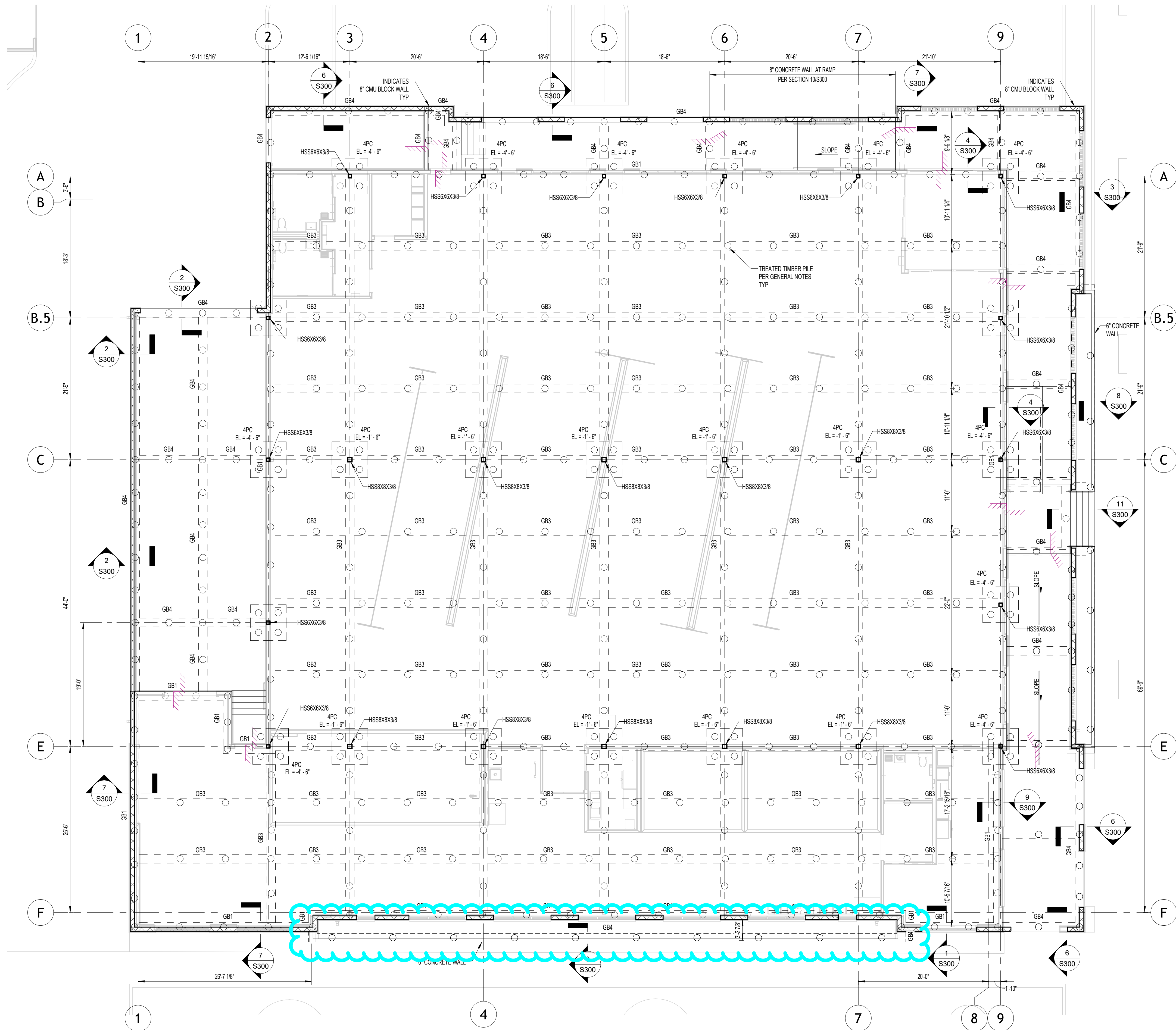
1 FOUNDATION PLAN 1/8" = 1'-0"
