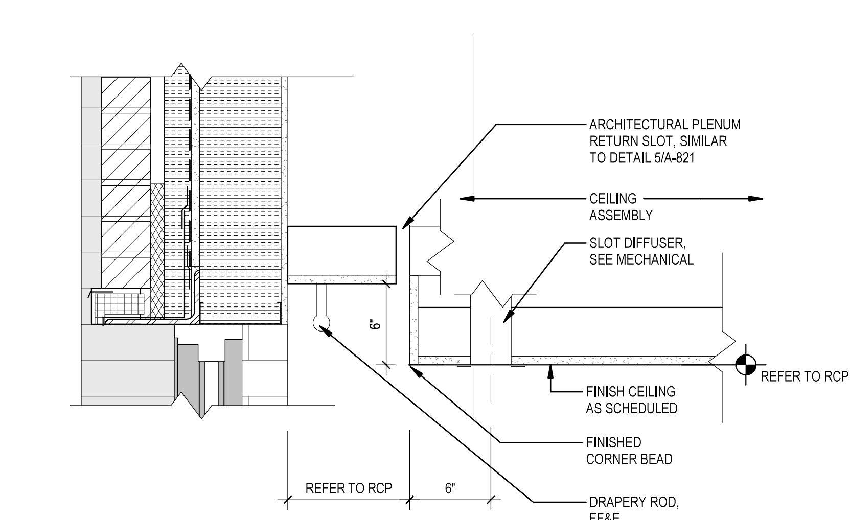
4 SECTION - WINDOW POCKET - AMENITY SCALE: 1 1/2" = 1'-0"
