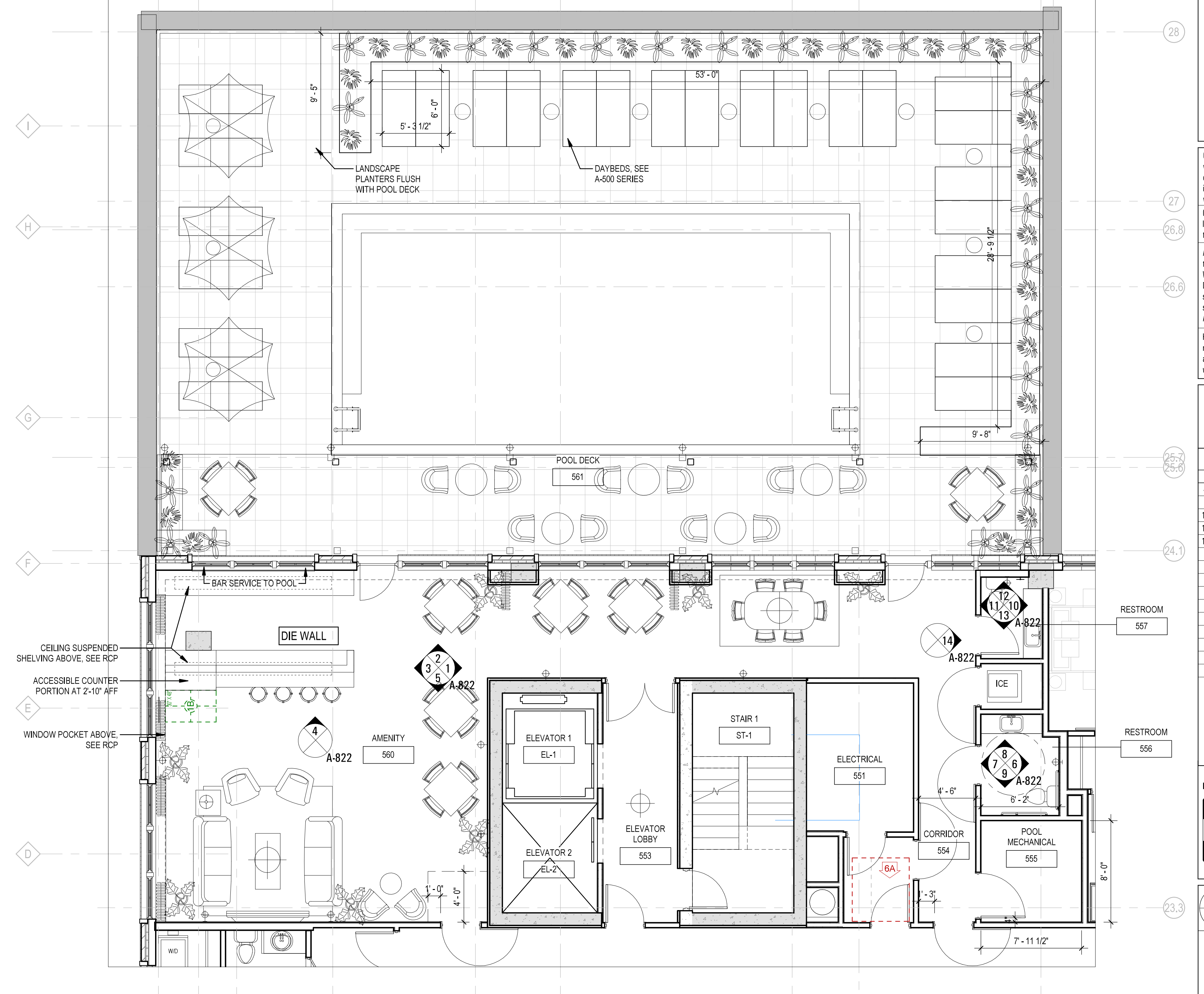
1 5TH FLOOR FURNITURE PLAN SCALE: 3/16" = 1'-0"
