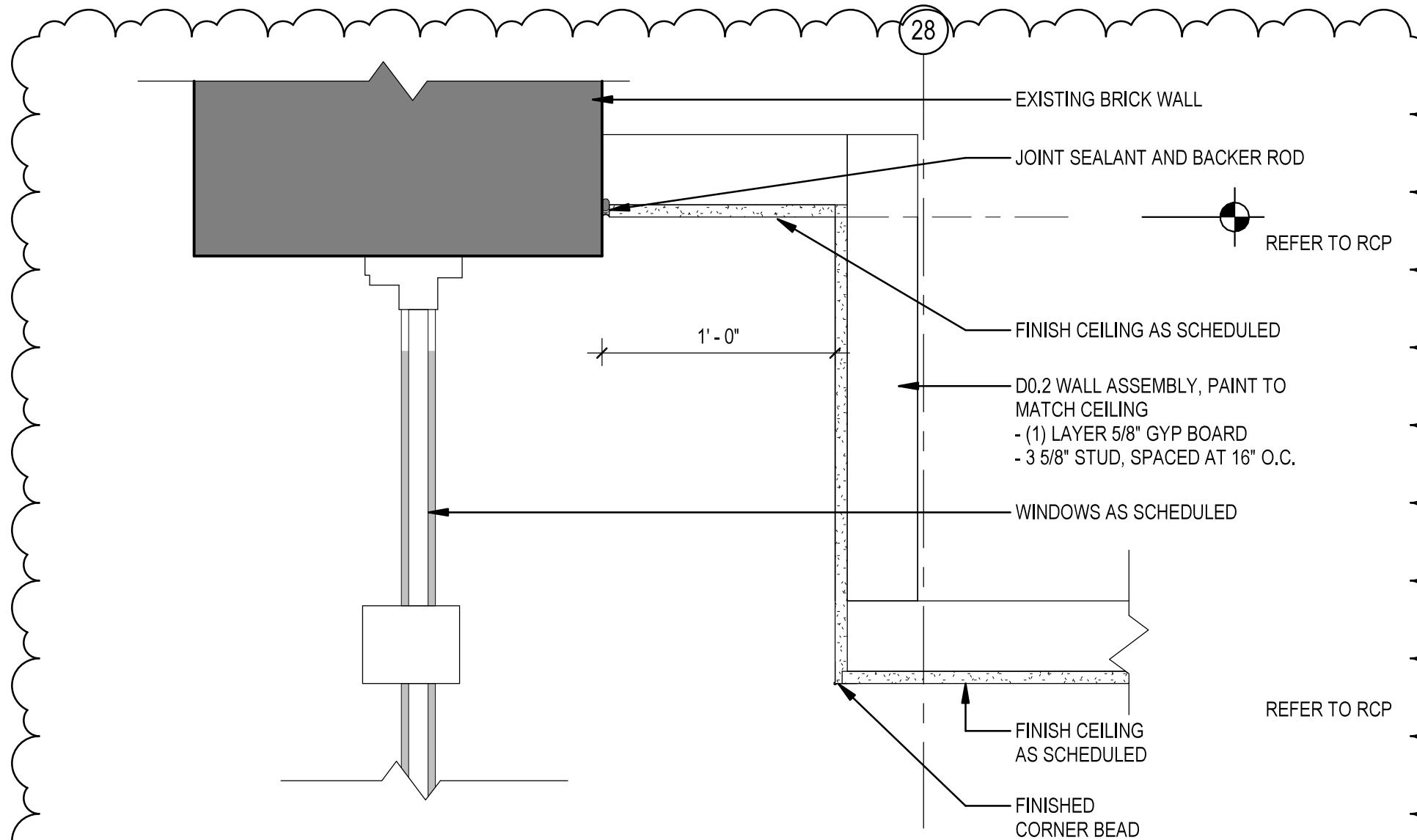
7 SECTION - TYPICAL WINDOW POCKET SCALE: 1 1/2" = 1'-0"
