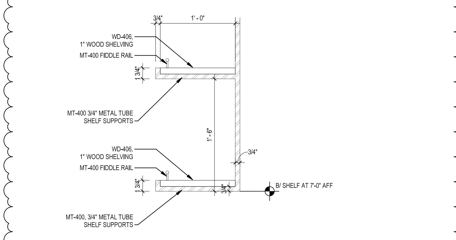
6 SECTION - SUSPENDED SHELVING SCALE: 1 1/2" = 1'-0"
