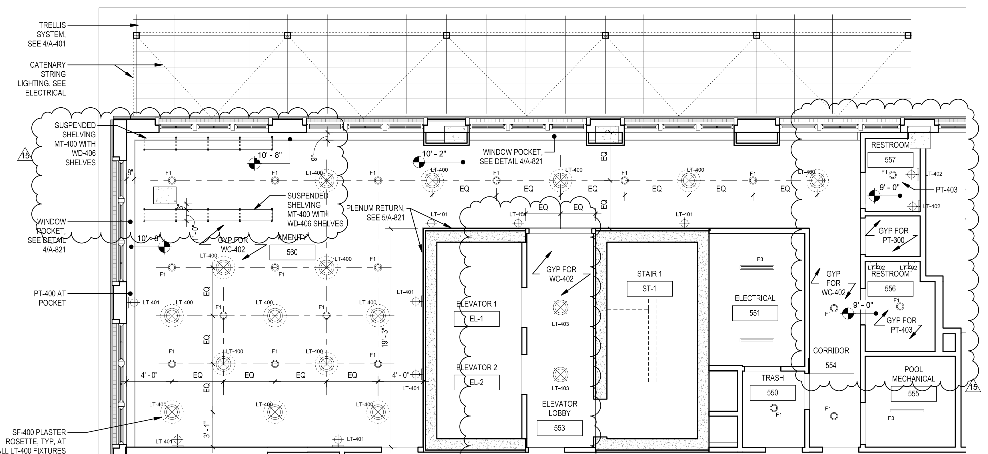
3 5TH FLOOR REFLECTED CEILING PLAN - INTERIOR SCALE: 3/16" = 1'-0"
