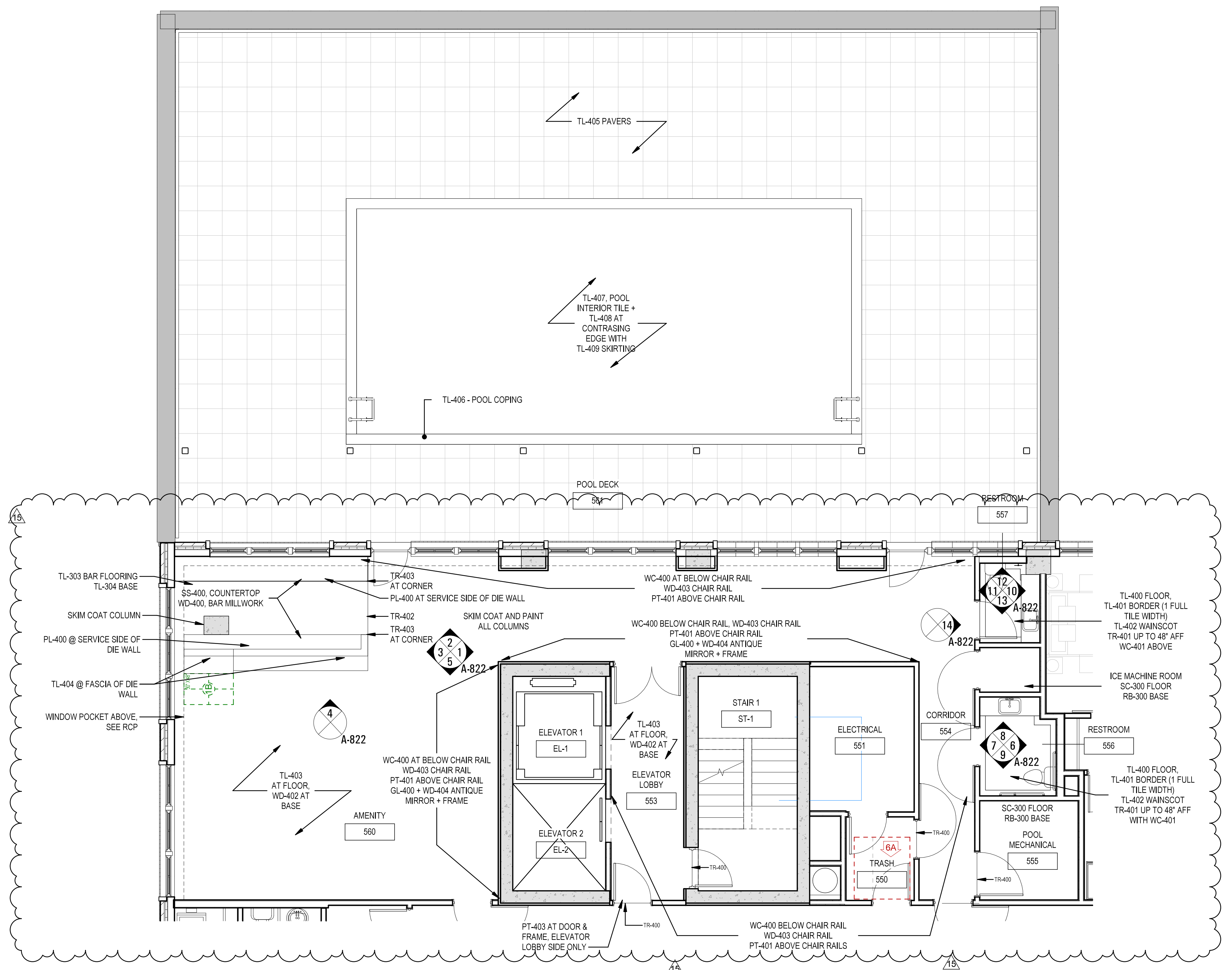
2 5TH FLOOR FINISH PLAN SCALE: 3/16" = 1'-0"
