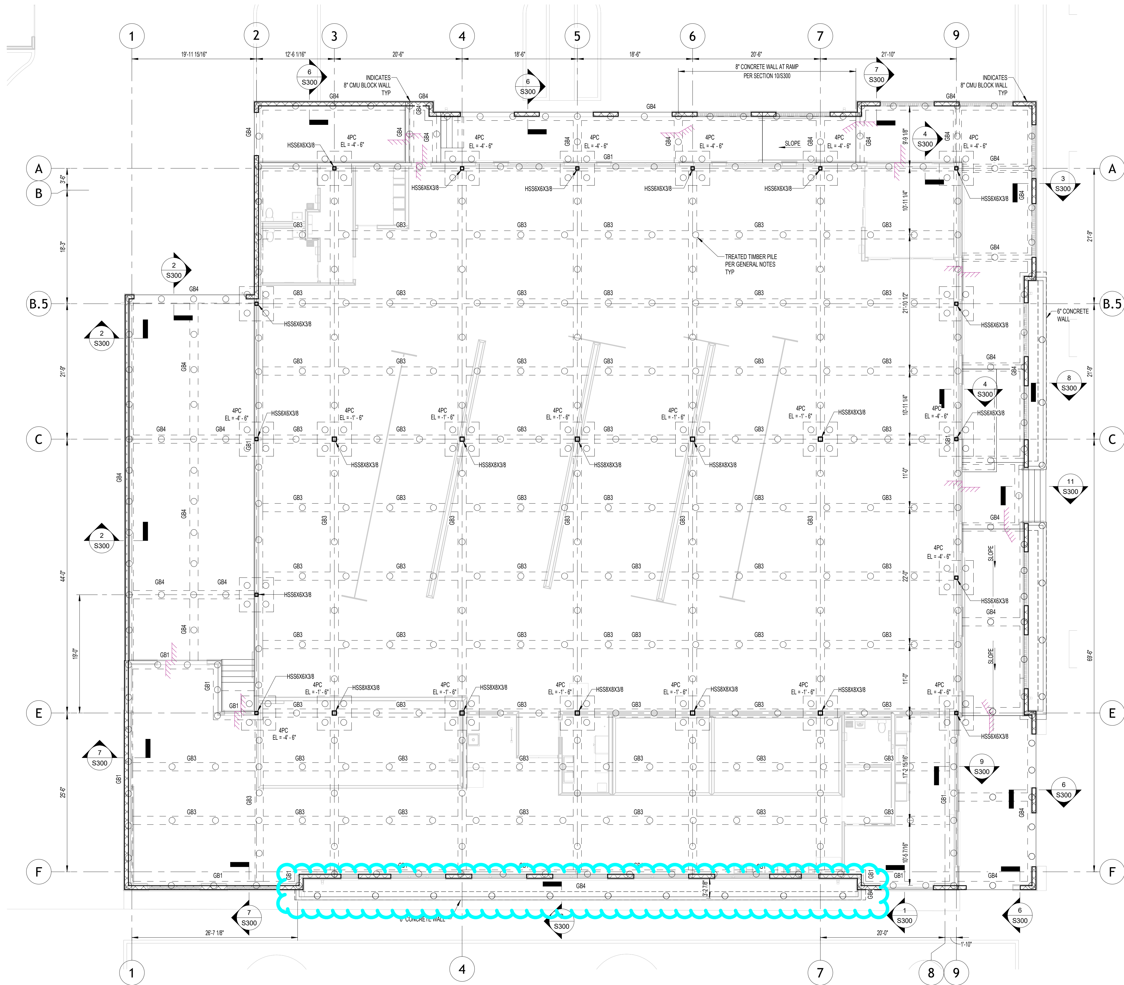
1 FOUNDATION PLAN 1/8" = 1'-0"
